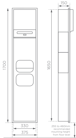
Automatic Tissue Roll Dispenser
